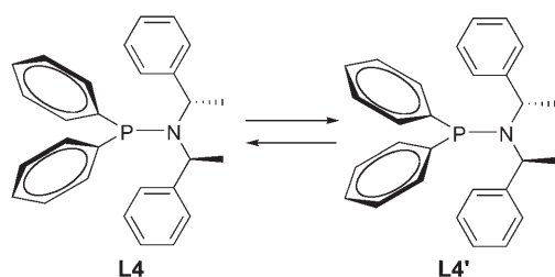
Scheme 3. Interconversion of helicity in L4 .
